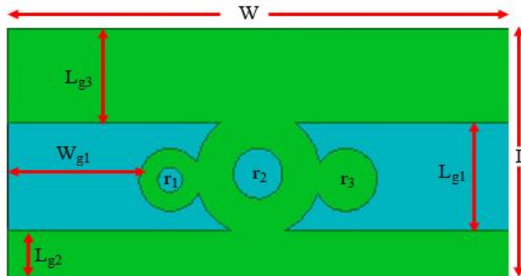
Fig. 2 Back plane
