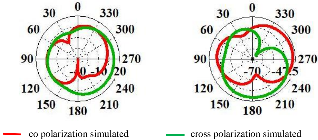
Fig. 10 Tri-band MIMO structure Radiation Patterns at 3.5 GHz, 5.5 GHz and 6.6 GHz
